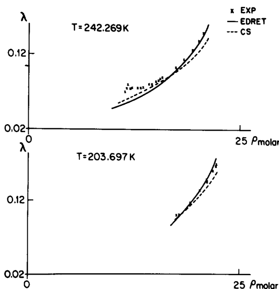
Fig. 5. Thermal conductivity in \text{W m}^{-1} \text{K}^{-1} , of a mixture of methane/ethane ( X_{\text{CH}_4} = 0.68526 ) versus the molar density.
