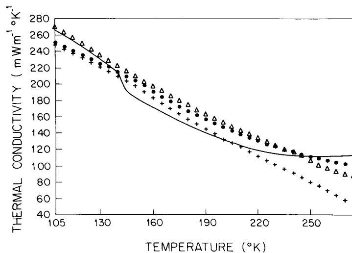
Fig. 3. Thermal conductivity, \lambda , of liquid ethylene versus temperature, at the saturation line. ( \Delta ) experimental; solid line, CSM; (+) EDRET without the internal degrees correction; ( \bullet ) EDRET with the internal degrees correction.
