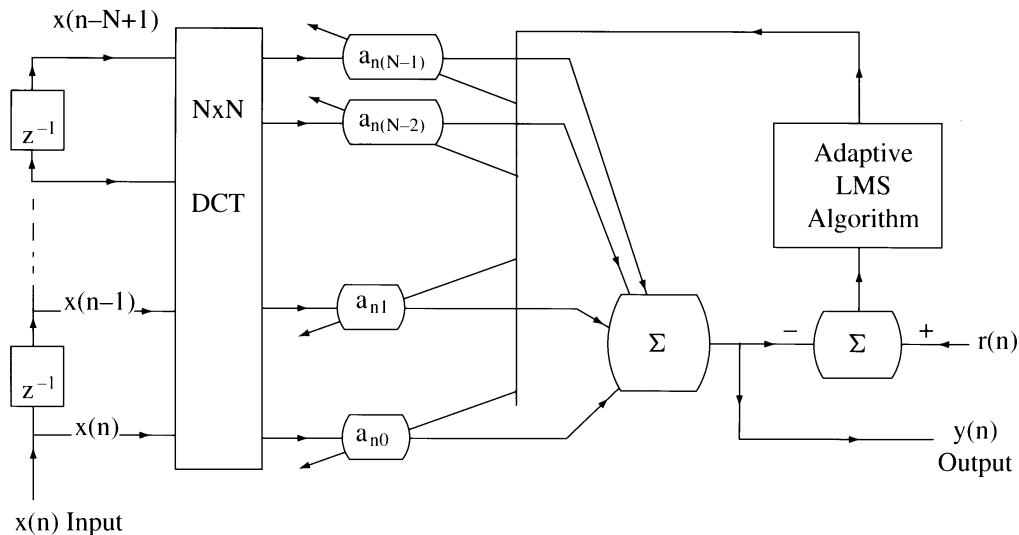
FIGURE 3.7 Adaptive transform domain LMS filtering.
