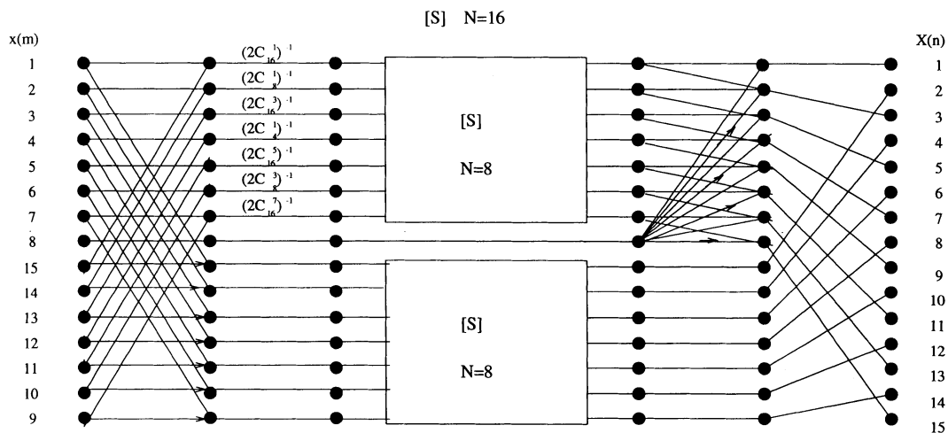
FIGURE 3.15 DIF DST N = 16 flow graph \rightarrow (-1) .
