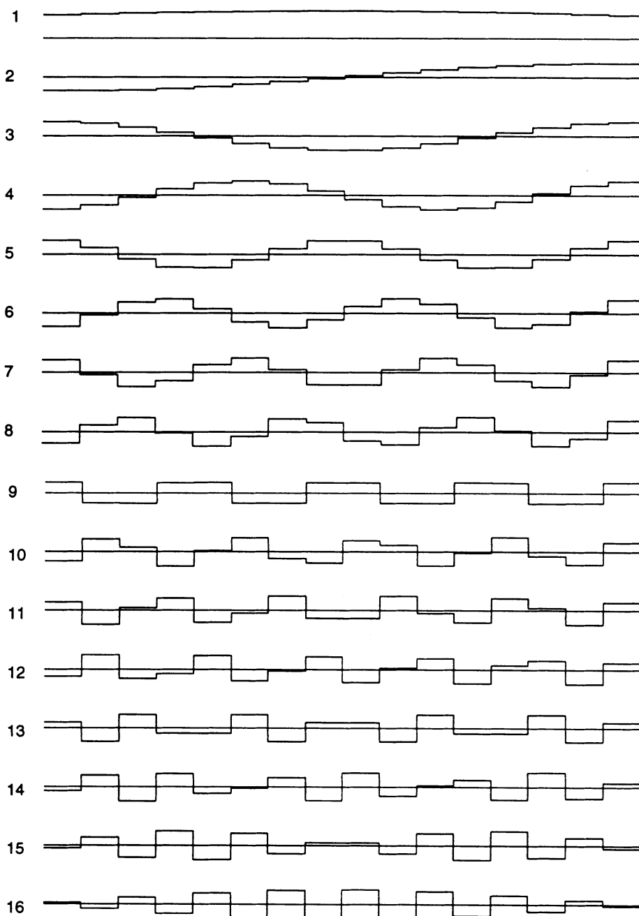
FIGURE 3.1 KLT Markov-1 signal \rho = 0.95 , N = 16 .
