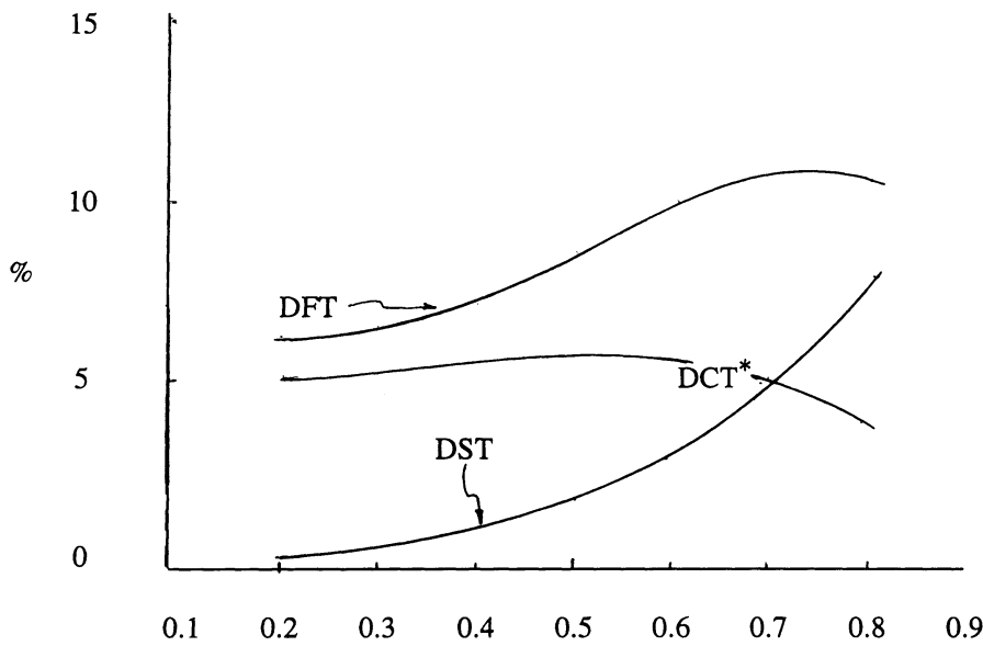
FIGURE 3.4 Percent Residual Correlation as a function of \rho, N = 16 .
