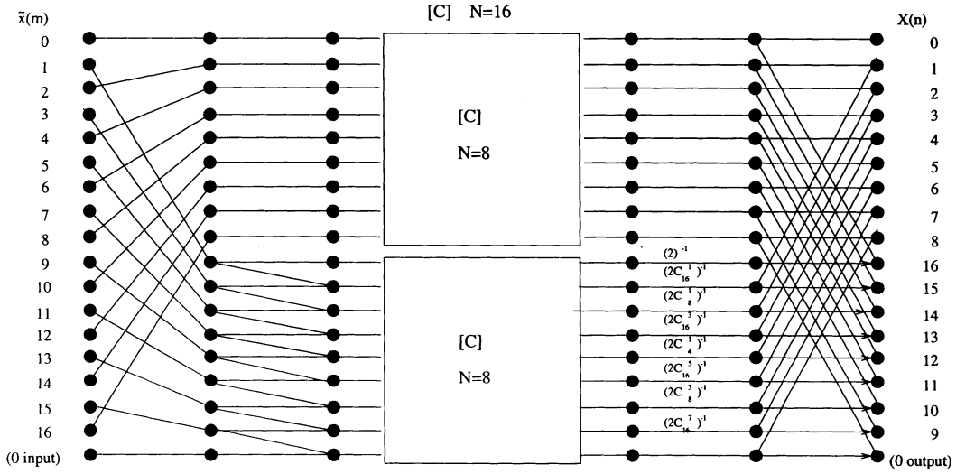
FIGURE 3.12 DIT DCT N = 16 flow graph \rightarrow (-1) .
