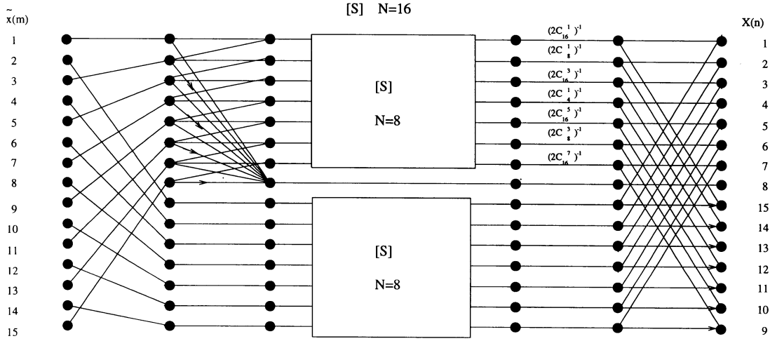
FIGURE 3.13 DIT DST N = 16 flow graph \rightarrow (-1) .
