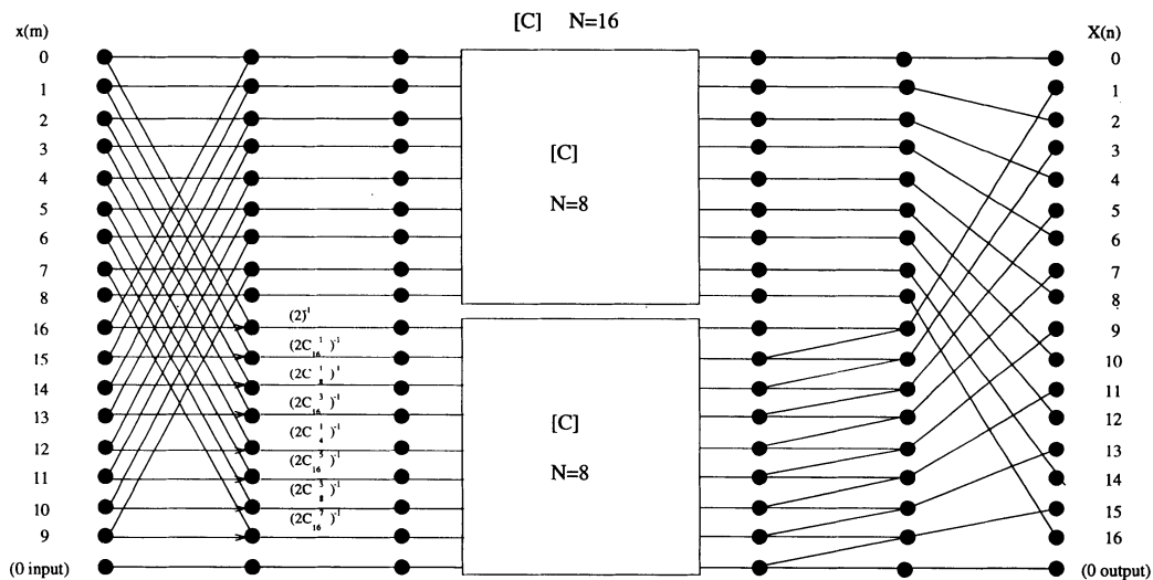
FIGURE 3.14 DIF DCT N = 16 flow graph \rightarrow (-1) .
